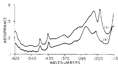
Figure 7. Fourier transform infrared absorption spectra of (a) (±)-mandelic acid [(±)-5] and (b) (±)-mandelic- \alpha -d acid [(±)-8] as 0.5 M solutions in dimethyl- d_6 sulfoxide.
